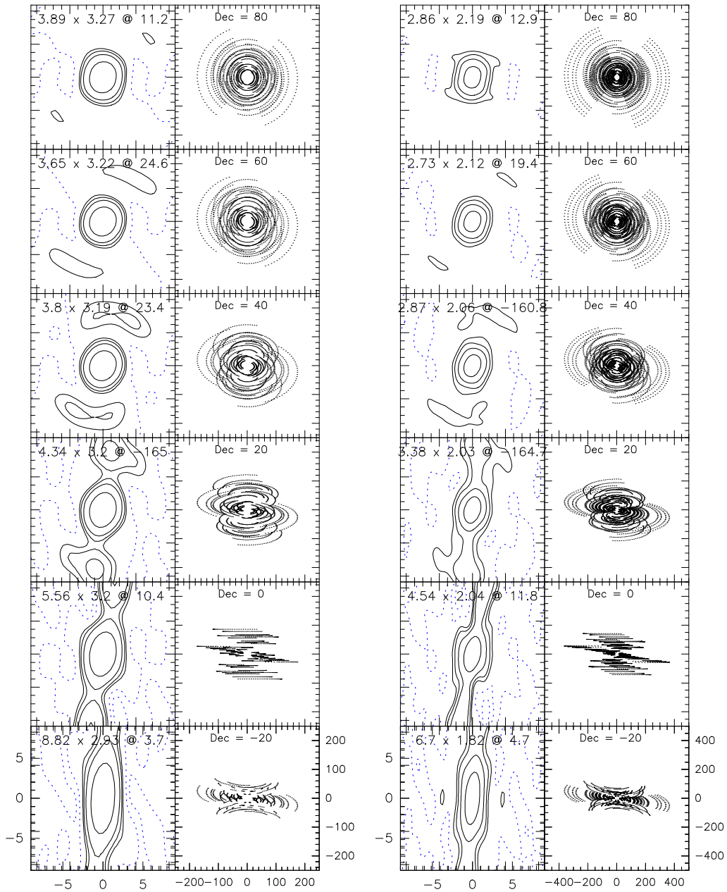
Figure 2: uv-plane coverage and beamshapes for the D and CD (8 antenna) configurations. Contour levels are at 5%, 10%, 20%, and 50%. Frequency is 100 GHz.
