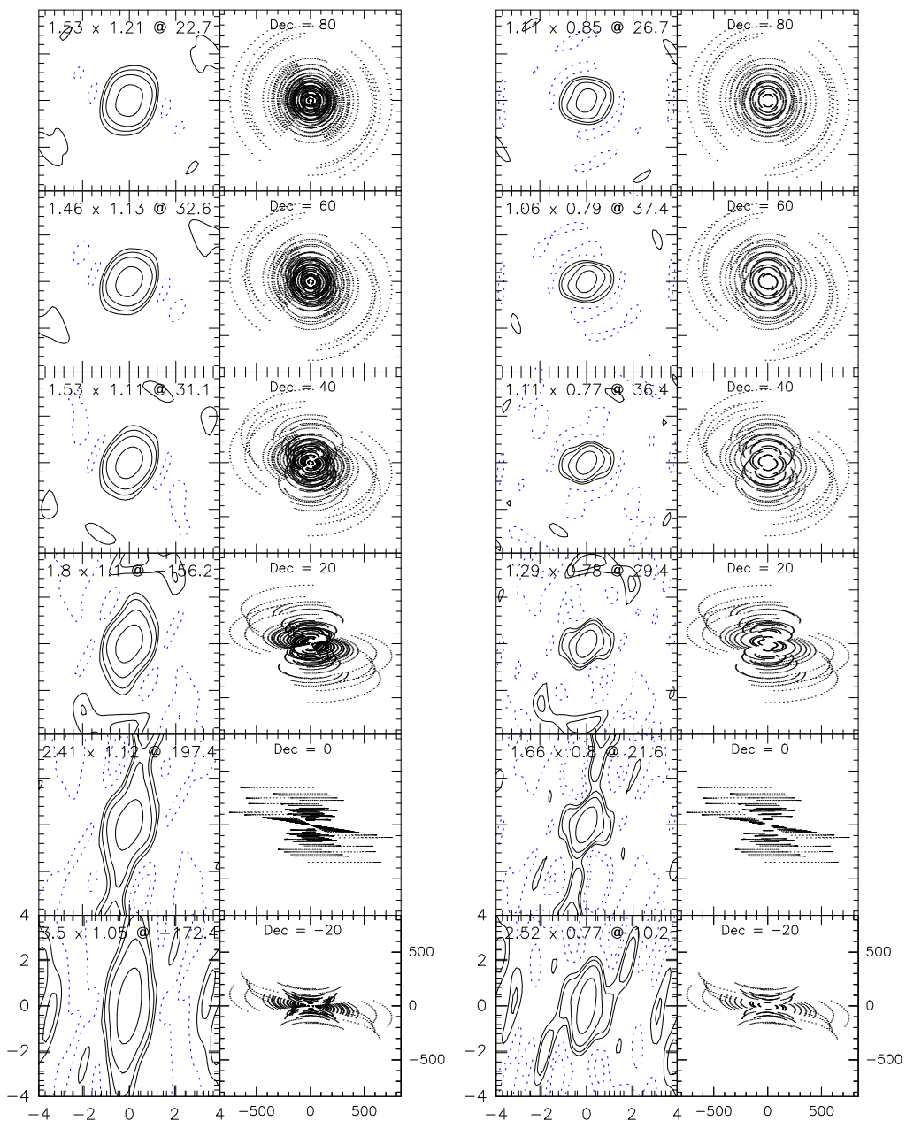
Figure 3: uv-plane coverage and beamshapes for the AC and A (8 antenna) configurations. Contour levels are at 5%, 10%, 20%, and 50%. Frequency is 100 GHz. Note the different scaling of the beam maps with respect to Fig. 2.
