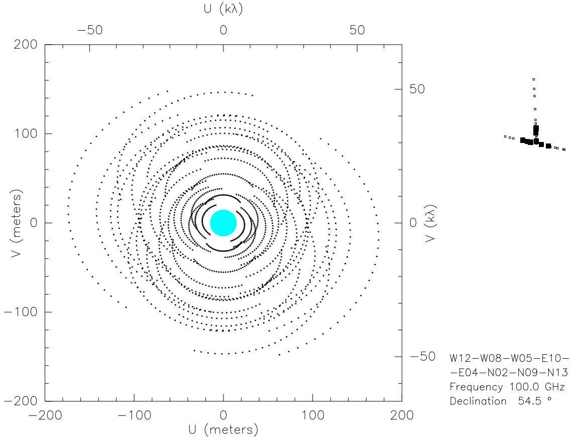
Figure 1: Example of uv-coverage (left) and interferometer station layout (right) for the 8D configuration, as produced by the ASTRO UV_TRACK command. The shaded circle at the center of the uv-plane shows the antenna shadowing region.
