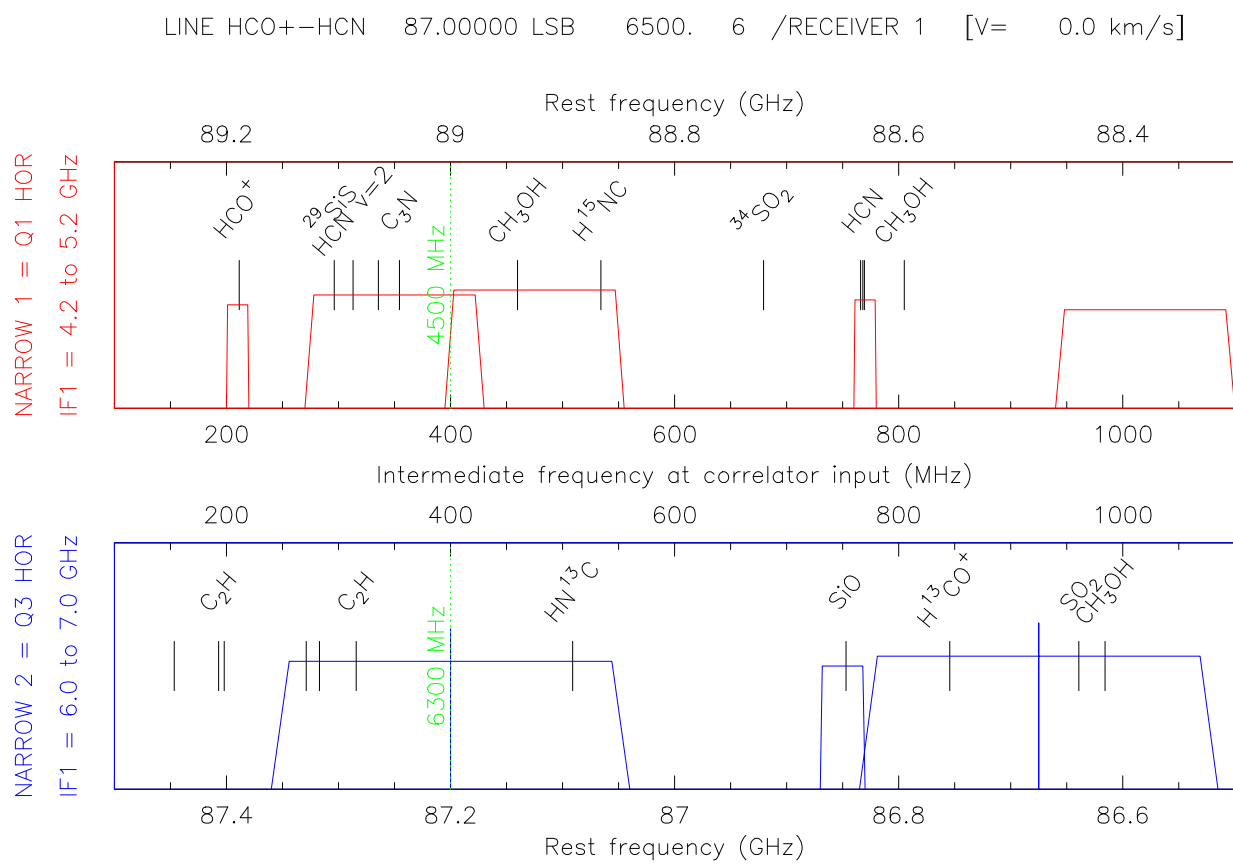
Figure 5: Example of spectral coverage by the narrow-band correlator, as produced by the ASTRO LINE command. Possible contamination by instrumental interferences are indicated in green.
