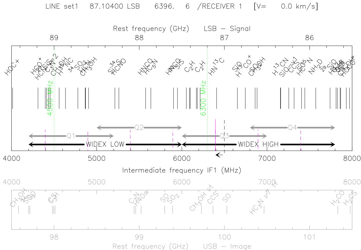
Figure 4: Example of spectral coverage as produced by the ASTRO LINE command (see Sect. 2.3.4). The image band is plotted for information only, the receivers are operated in single side band mode. Possible contamination by instrumental interferences in the signal band are indicated in green. IF frequencies respecting the 500 MHz spaced tuning grid are indicated by dashed magenta lines. The IF frequency on which the tuned sky frequency is centered, is shown by a magenta solid line
